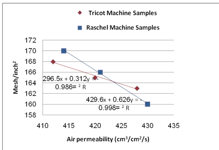
Figure 6 The Relation Between Air Permeability (cm³/cm²/s) and Mesh Density (Mesh/inch²)
