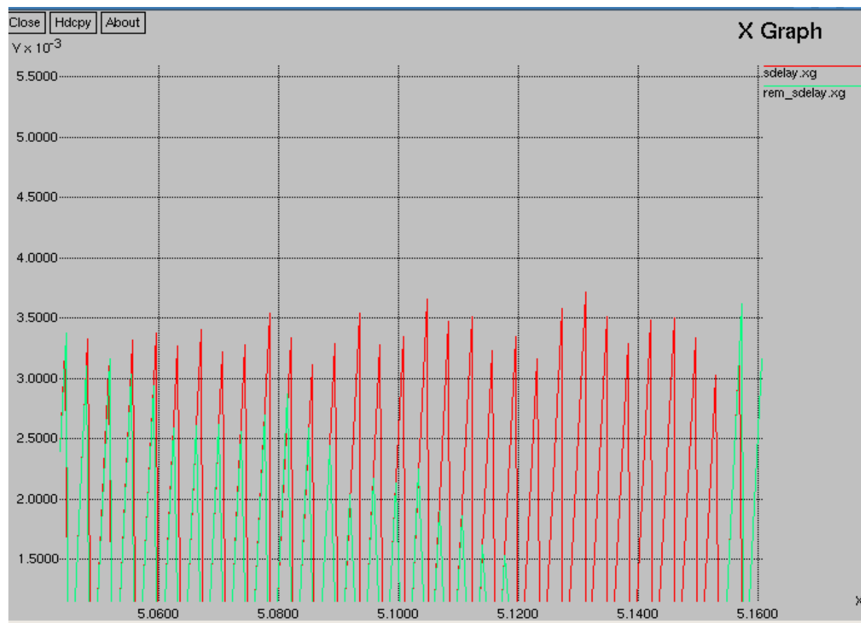
Fig 2: Delay
