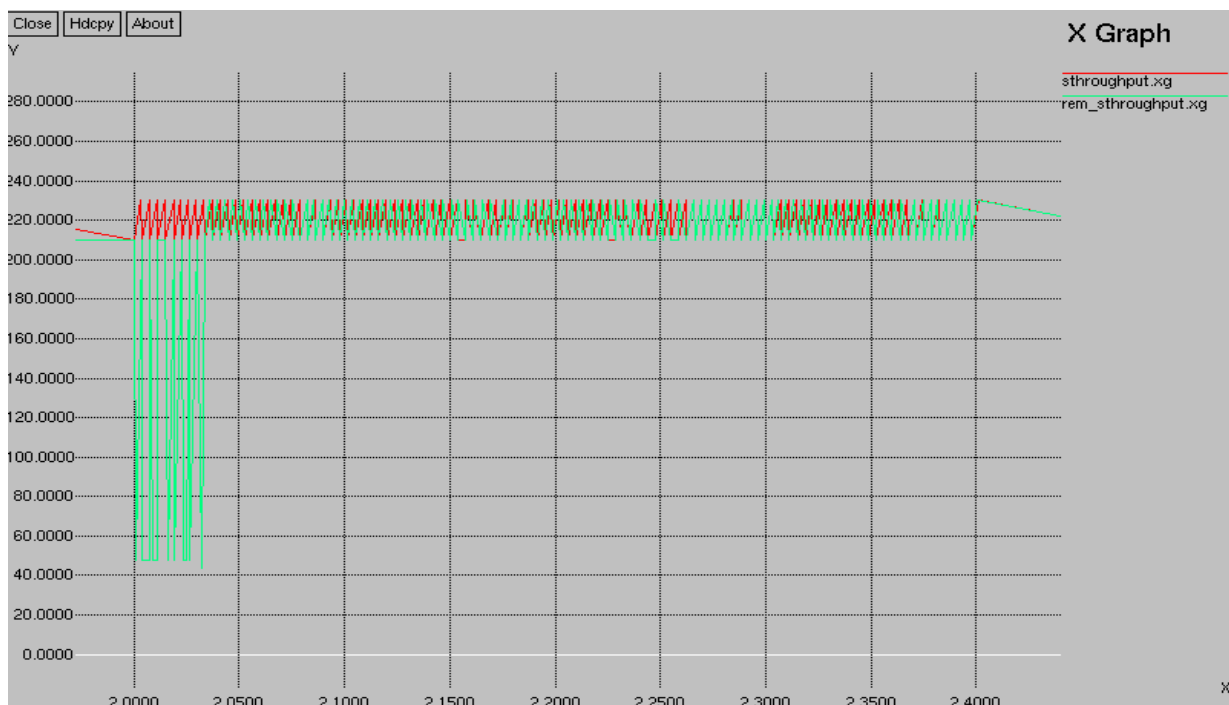
Fig 4: Throughput
