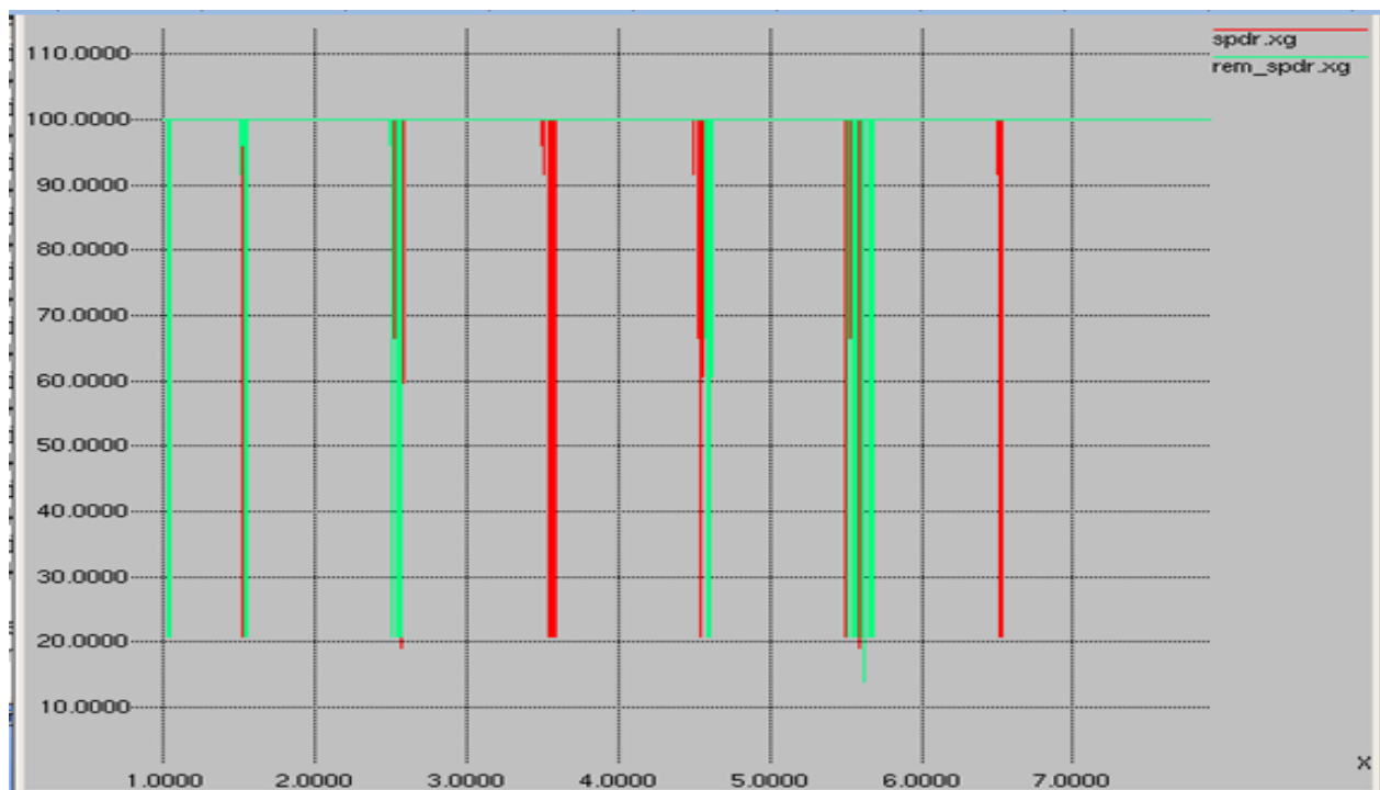
Fig 3: PDR
