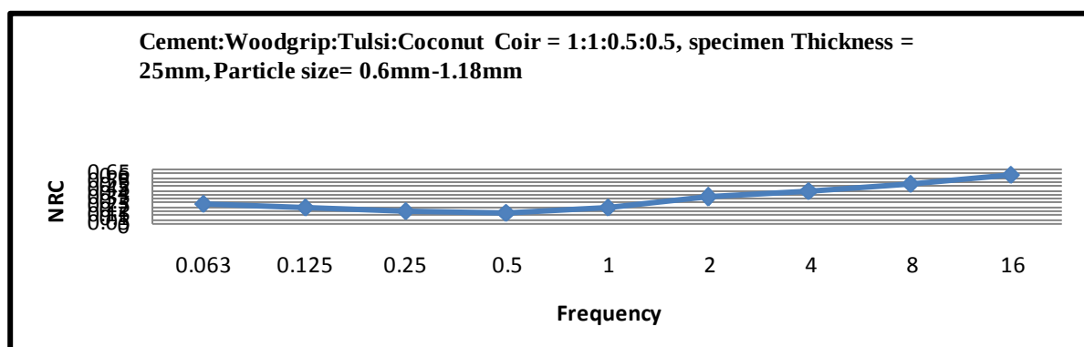
Fig. 4 Graph of Cement:Woodgrip:Tulsi:Coconut coir Showing NRC
