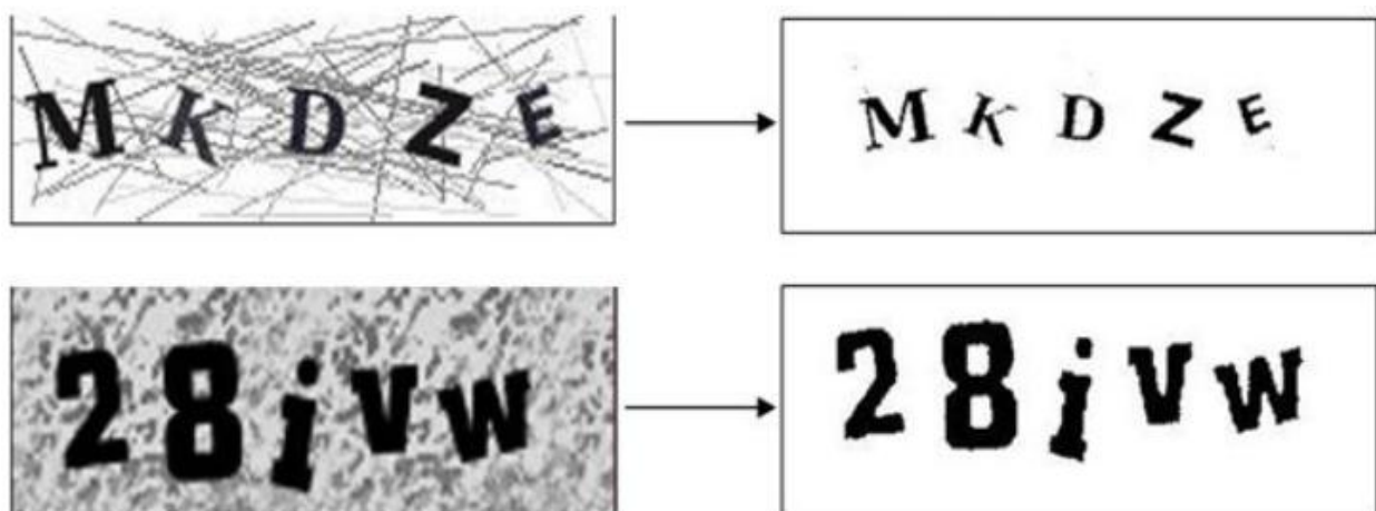
Fig.5: Segmentation result for captcha
