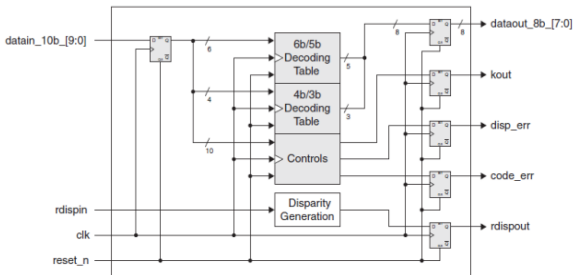
Fig2: Receiver block
