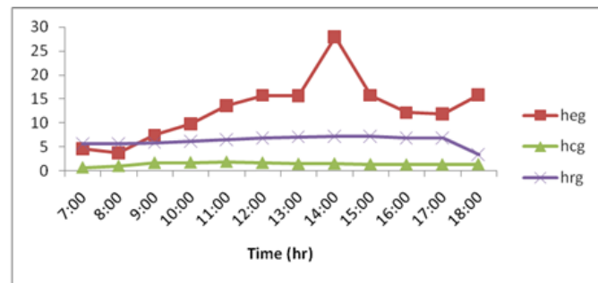
Figure 7: Variation of Various Heat Transfer Coefficients For Weir Type Stepped Solar Still
