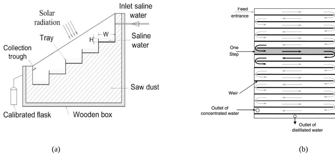
Figure 2 (A, B): Schematic View Of Stepped Solar Still and Absorber Plate of Weir Type Solar Still
