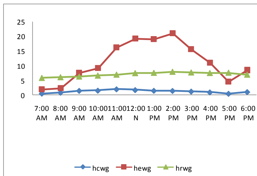
Figure 6: Variation of Various Heat Transfer Coefficients For Stepped Solar Still
