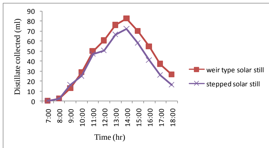
Figure5. Distillate output of stepped and weir type solar still
