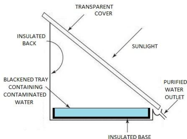
Figure 1. Schematic view of conventional solar still
