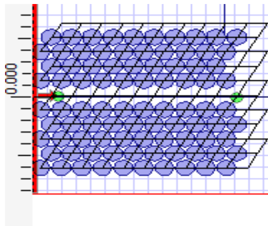
Fig 4(a) Waveguide bounded by circular unit cell with refractive index-2.94.
