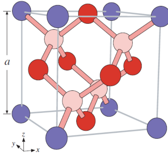
Figure 3: Structure of Three-Dimensional Photonic Crystal [6]
