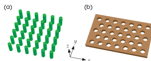
Figure 2:(a) Schematic of a 2D rod-type Photonic crystal consisting of high refractive index cylinders in a low-index background (b) Schematic of a 2D hole-type Photonic crystal slab consisting of low refractive index cylinders in a high-index slab[5]
