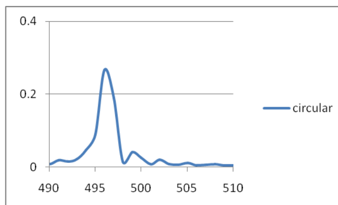
Fig 6.(a) Power measured at output of waveguide(refractive index-2.94).
