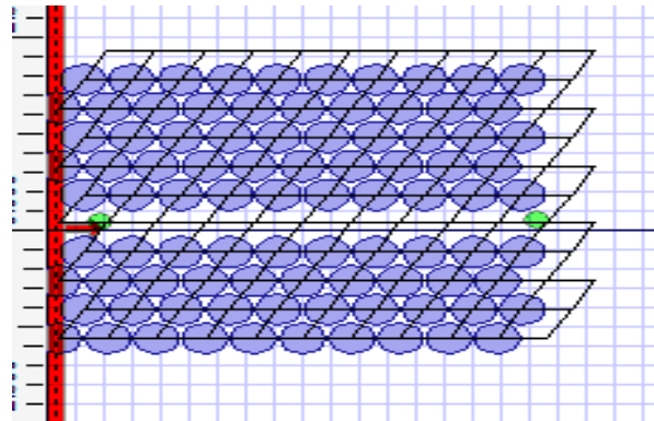
Fig-5(a) Waveguide bounded by circular unit cell with refractive index-3.45.
