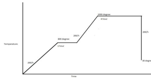
Fig.2.0 Sintering cycle
