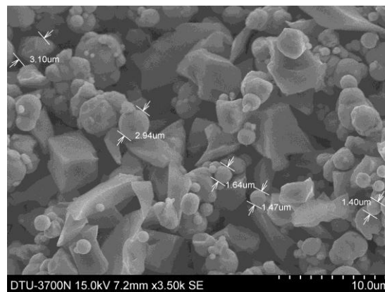
Fig. 2.1 SEM micrograph of unbonded magnetic abrasive particles
