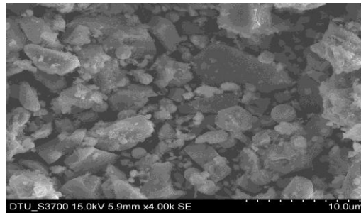
Fig 2.4 SEM micro graph of sintered magnetic abrasive particles
