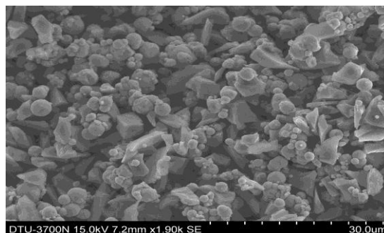
Fig. 2.2 SEM micrograph of unbonded magnetic abrasive particles
