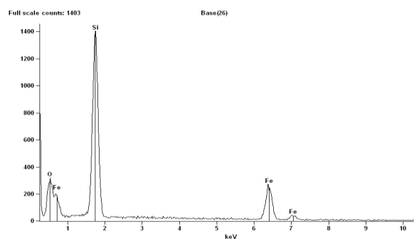
Fig. 2.6 EDS graph of solid sintered sample
