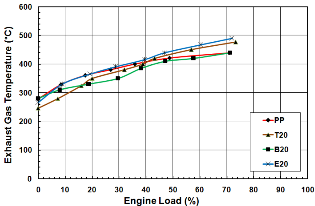
Fig. 4. Exhaust gas temperature Vs % engine load.
