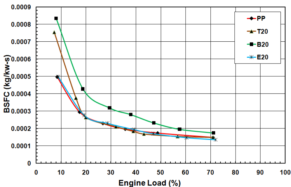
Fig. 2. BSFC Vs % engine load.
