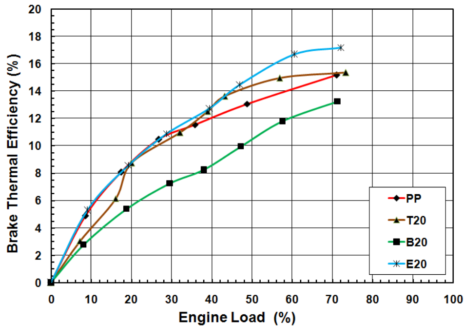
Fig. 3. Brake thermal efficiency Vs % engine load.
