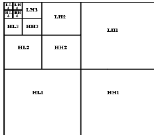
Figure 1: Four-Level Wavelet Decomposition.
