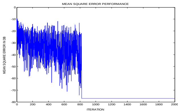
Fig.6 30 dB de-noised. Mean square error (dB) plots for 2000 iteration.
