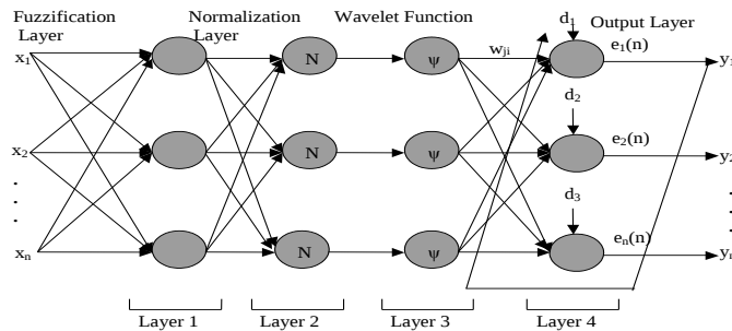
Fig.3 Fuzzy wavelet neural network model
