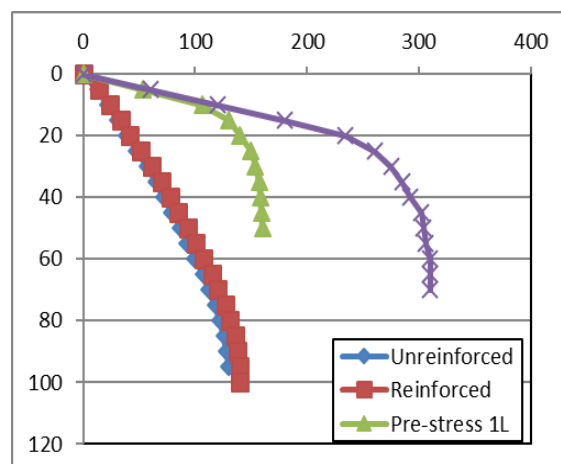
Fig. 8 Stress settlement relation for unreinforced, reinforced and pre-stressed cases at (Df/B = 1.0)
