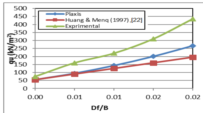
Fig. 7 Ultimate (B.C.) for different (Df/B) for reinforced soil without pre-stress
