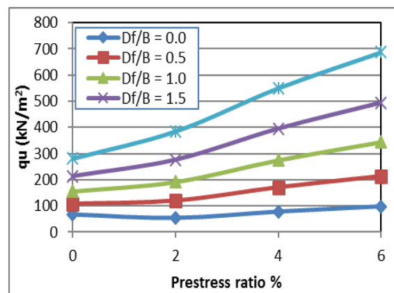
Fig. 10 Ultimate (B.C.) (qu) for different pre-stressing ratios (PS%) of double reinforcement layers (2LPs).
