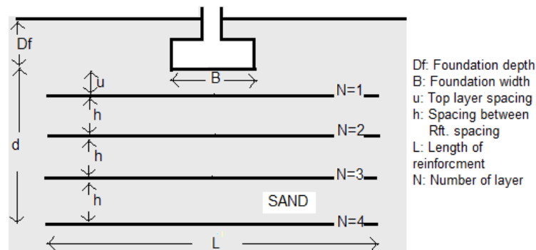
Fig. 4 Configuration of reinforcement layers
