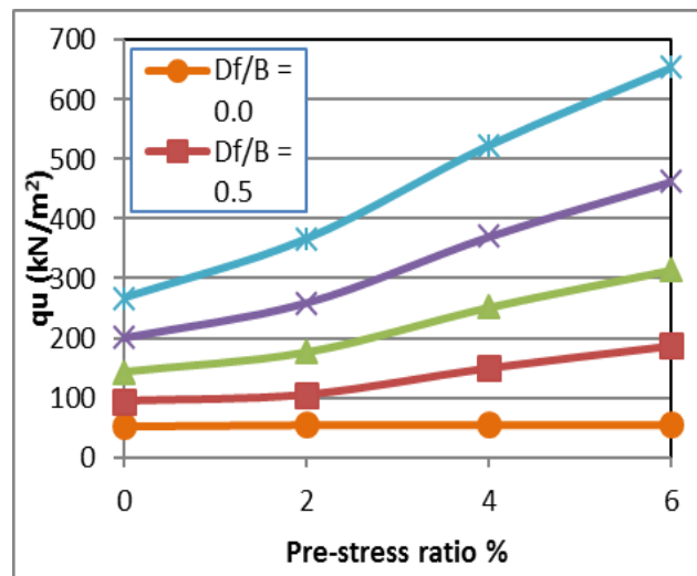
Fig. 9 Ultimate (B.C.) ( qu ) for varying pre-stressing ratios (PS%) of one reinforcement layer (1LPs).
