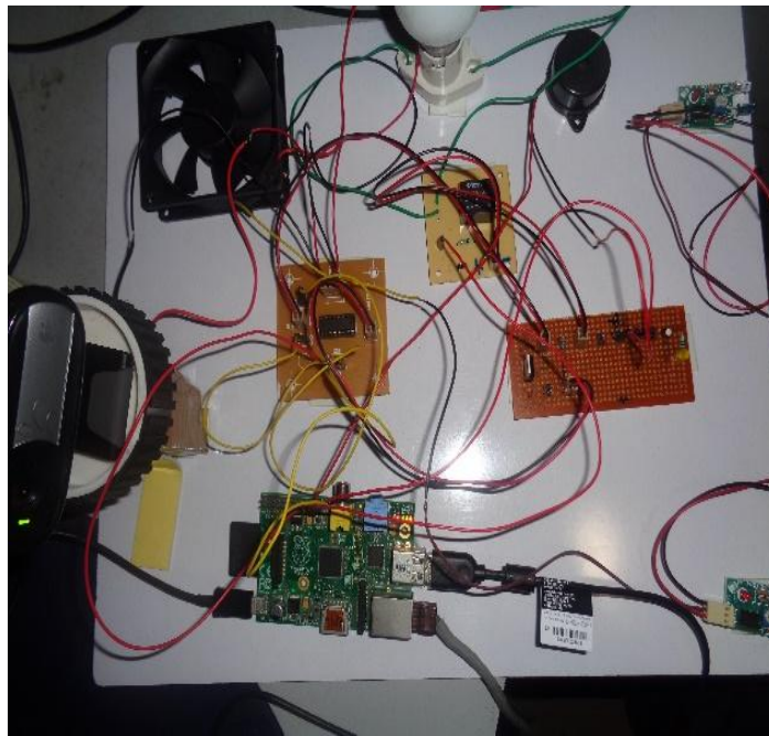
Fig3. System Design
