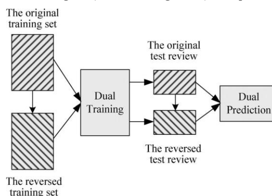
Fig.1. Process of dual sentiment analysis.
