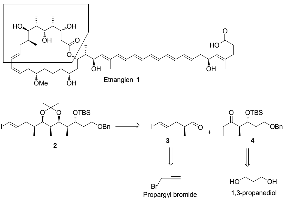
Fig 1: Retro Synthetic Analysis
