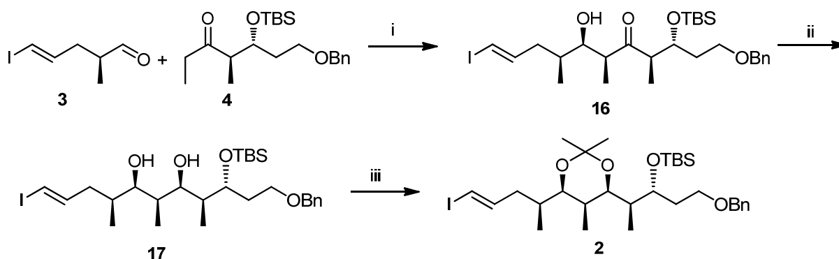
Fig 4: Coupling of aldehyde 3 ethyl ketone 4.
