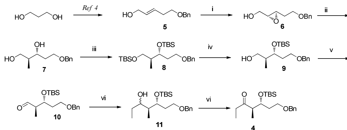
Fig 2: Synthesis of Fragment 4
