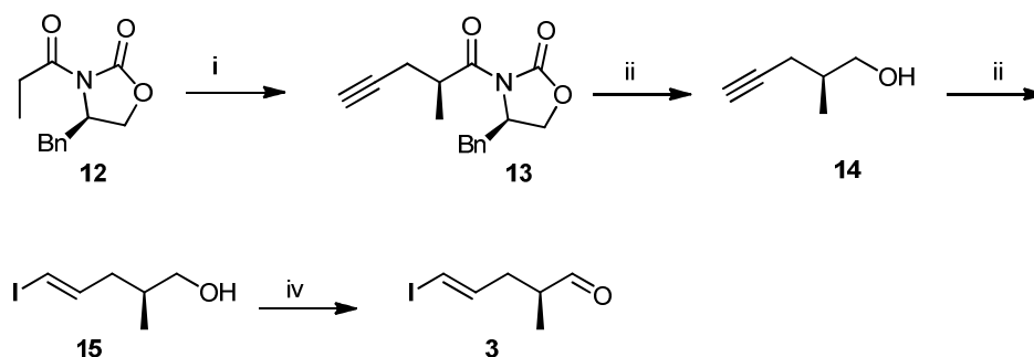
Fig 3: Synthesis of Aldehyde 3
