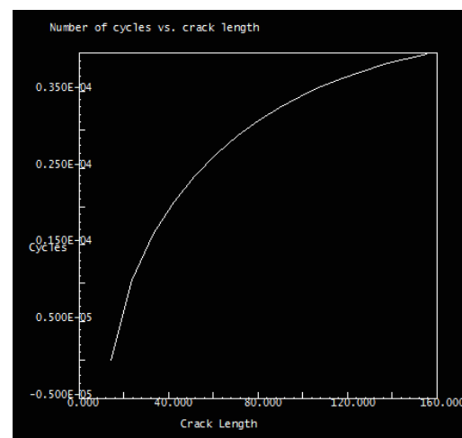
Figure 6. Crack length vs. no. of cycles for steel plate with rectangular cut outs 300mm apart
