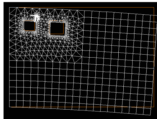
Figure 6. Finite Element Mesh of deformed shape After crack propagation
