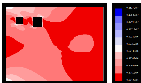
Fig 9. Von Mises Stress for steel plate with rectangular cut outs 200mm apart
