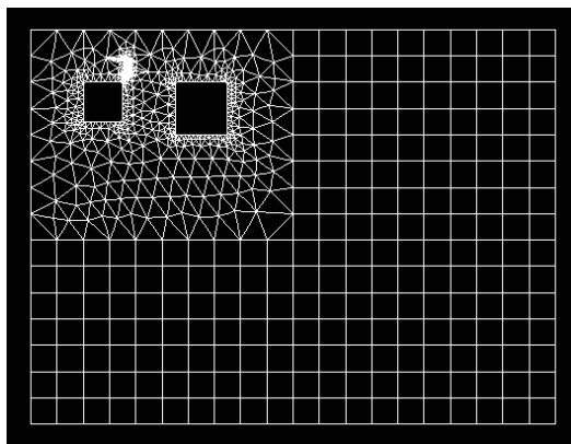
Figure3. Finite Element mesh of Crack at corner of cut out shape
