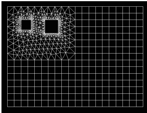
Figure 1. Finite Element Mesh of Steel Plate
