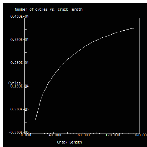
Fig 7. Crack length vs. no. of cycles for steel plate with rectangular cut outs 400mm apart
