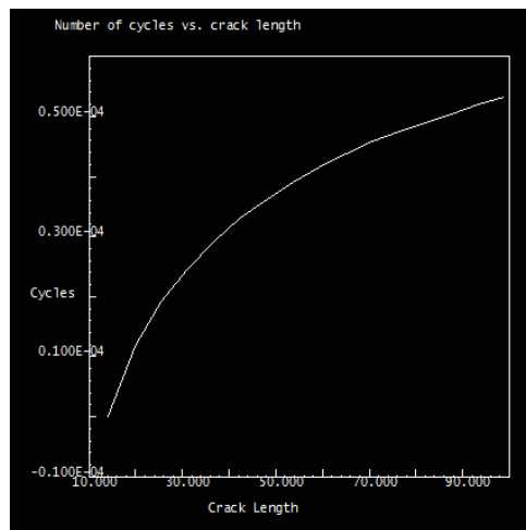
Figure 5. Crack length vs. no. of cycles for steel plate with rectangular cut outs 200mm apart
