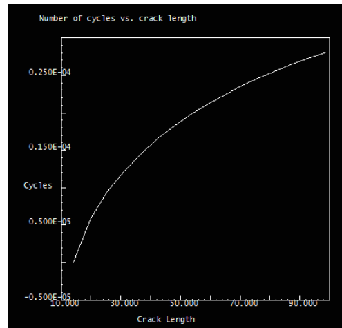
Fig 8. Crack length vs. no. of cycles for steel plate with rectangular cut outs 500mm apart
