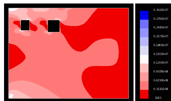
Fig 10. Von Mises Stress for steel plate with rectangular cut outs 300mm apart
