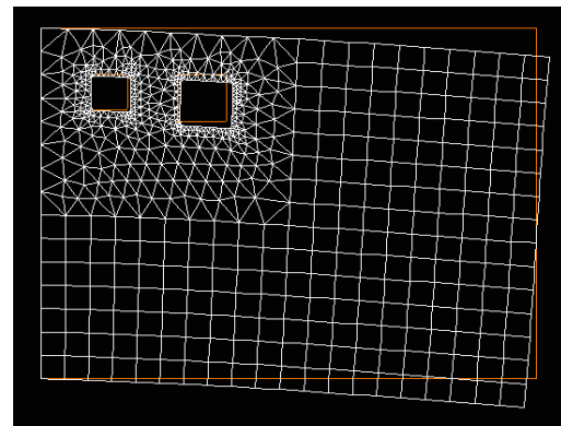
Figure2. Finite Element Mesh of Deform Shape with rectangular cut out of Steel Plate
