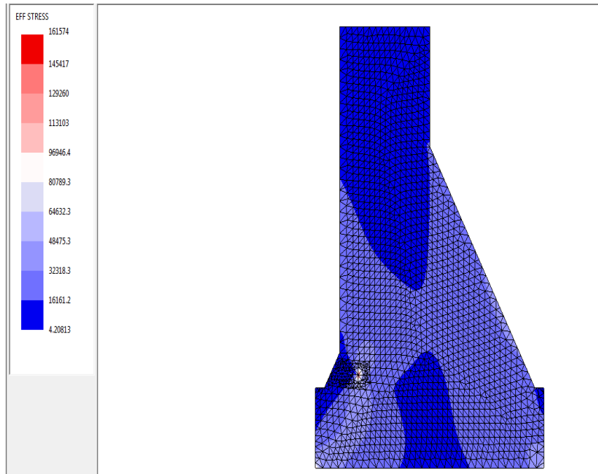
Fig. 2.9. Effective stress values after the application of the crack for water flowing at the height three meter greater than that of the height of the dam.
