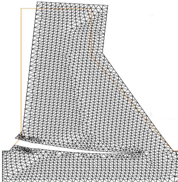
Fig.2.8. Deformed mesh after the application of crack for the water flowing at three meter height greater than that of the dam
