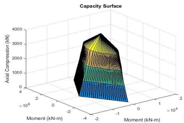
Fig. 4.4 Capacity Surface for case-2
