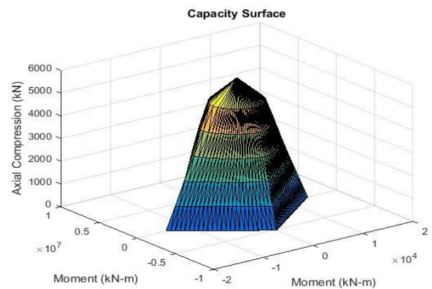
Fig. 4.6 Capacity Surface for case-3
