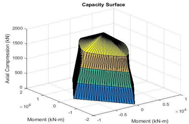
Fig. 4.2 Capacity Surface for case-1
