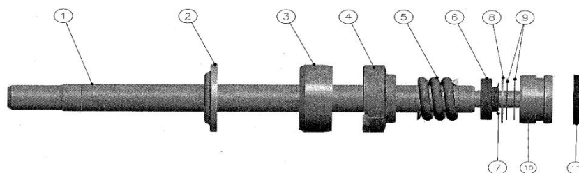
Fig.Piston rod assly
