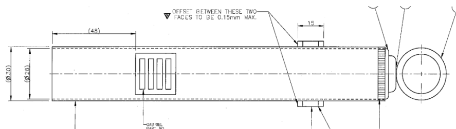
Fig. Outer tube assly
