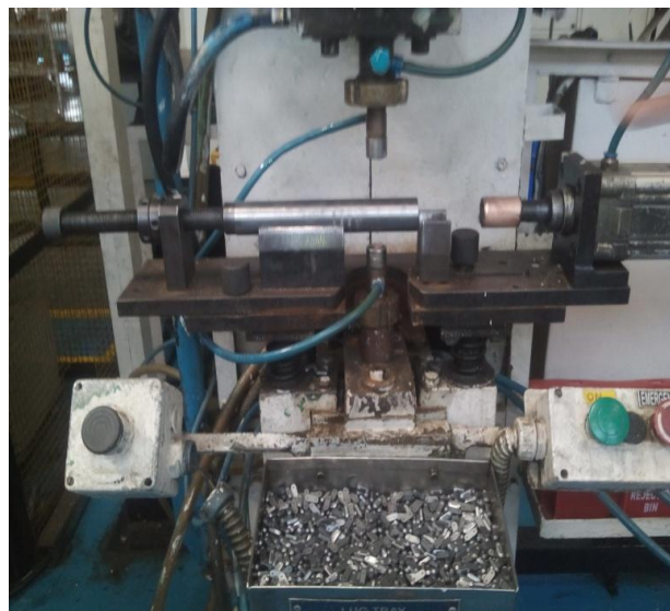
Fig.3.1:Lug Welding machine
