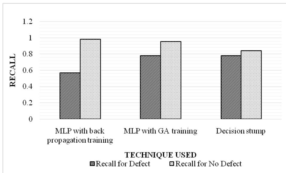
Figure 4 Recall
