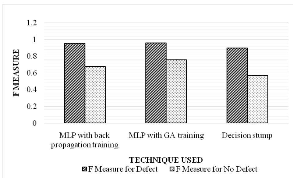
Figure 5 F Measure
