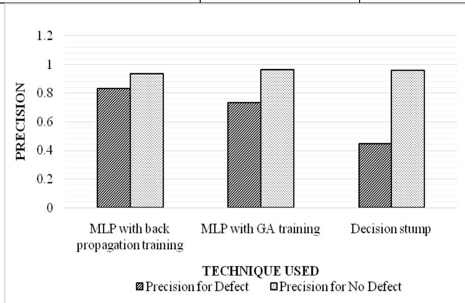
Figure 3 Precision
