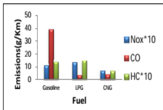
Fig 2 A Summary of Emission with Non-Catalyst Vehicle
