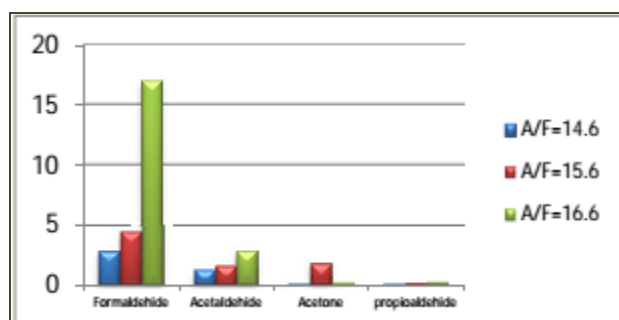
Fig 4 Concentration (ppmv) of aldehydes in exhaust gases of LPG fuelled engine.
