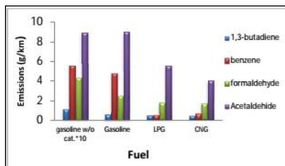
Fig-3 Unregulated emission components different fuel
