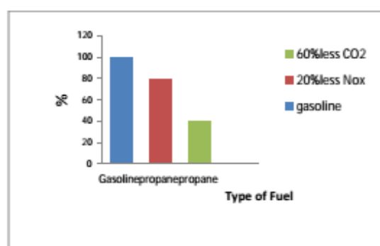
Fig.1 Vehicle Emissions
