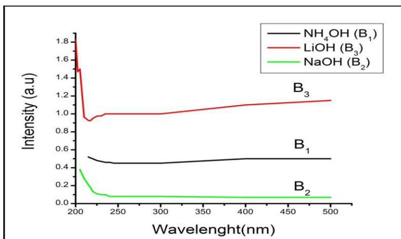
Fig. 2 UV-Visible absorption spectra of ZnO nanostructures prepared with (a) \text{NH}_4\text{OH} (b) Li(c) NaOH.
