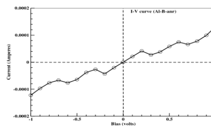
Fig 4: I-V characteristic curve of AlBnanr showing current in the forward and reverse bias region.
