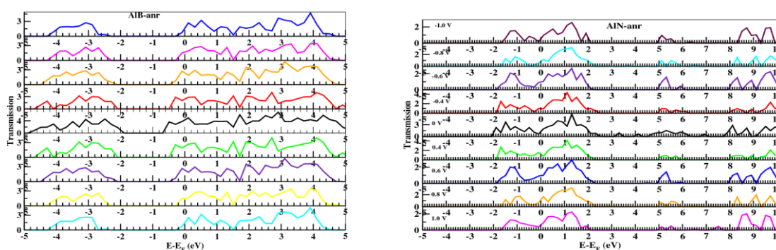
Fig6: Transmission curves of AlB-anr and AlN-anr
