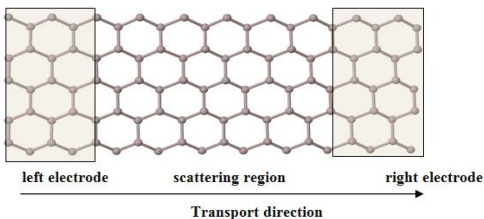
Fig 1: Schematic structure of the model device constituted by three parts: the left (L) and right (R) semi-infinite Al 1 Zn 1 R (electrodes) and scattering region
