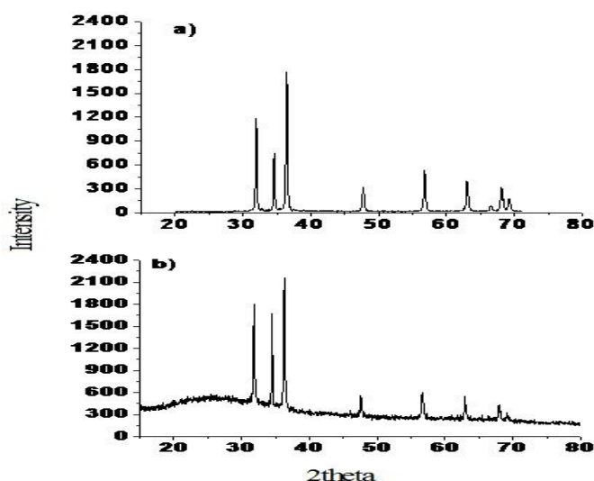
Figure 1: XRD pattern of (a) ZnO NPs and (b) ZnO NWs
