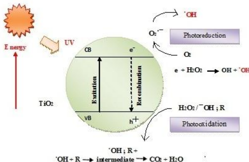
Figure 4: Mechanism of photocatalysis activity [31]
