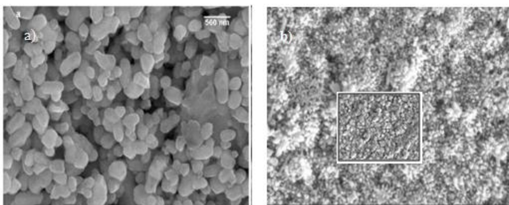
Figure 2: SEM image of ZnO thin film a) Spherical shape ZnO NPs and b) ZnO NWs.
