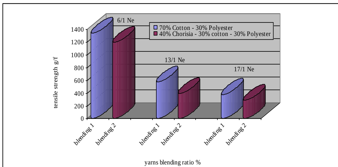
Figure 1. The effect of blending on the tensile strength g/f of yarns
