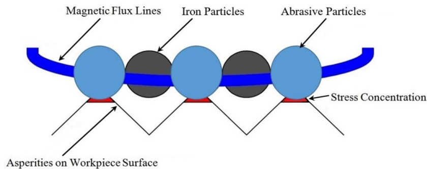
Fig. 1 Plausible Mechanism of Wearing of Asperities in Magneto Rheological Finishing Process
