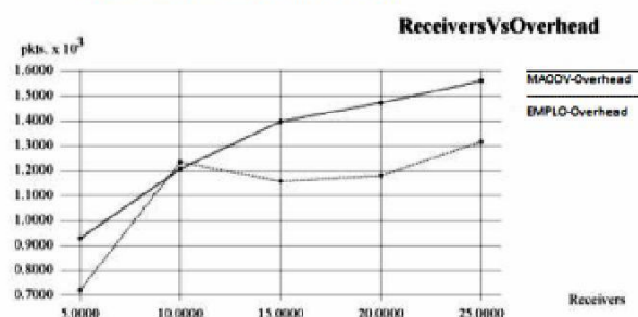
Fig. 12. Overhead as a Function of Receivers
