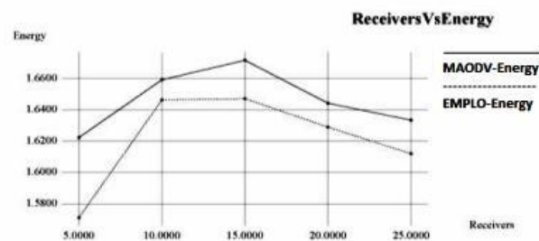
Fig. 9. Energy Consumption as a Function of Receivers
