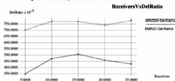
Fig. 11. Delivery Ratio as a Function of Receivers
