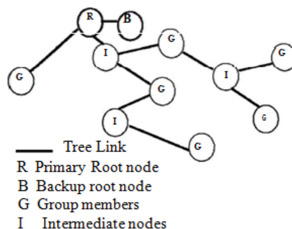
Fig :1 Shared Multicast Tree with Backup Root
