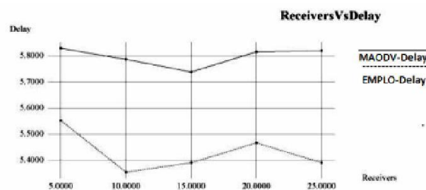
Fig. 10. End-to-End Delay as a Function of Receivers
