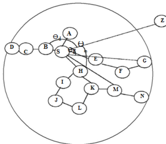
Fig.2. 3 Hop Routing zone at node S
