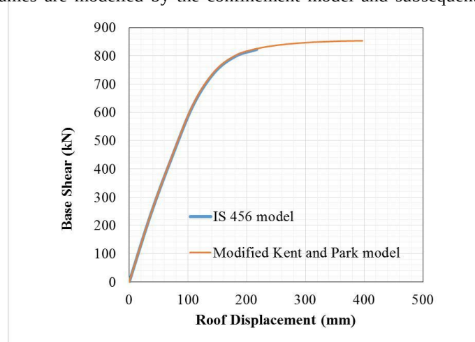
Fig: 8 Effect of confinement in lateral load behaviour of 12 storeyed SMRF frames
