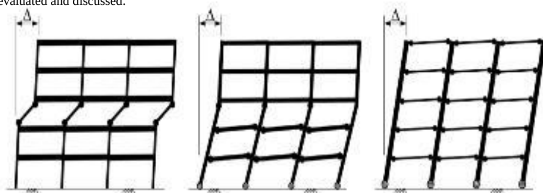
Fig: 4: Story mechanism Intermediate mechanism Beam mechanism (Reference: Moehle et al. , 2008)
