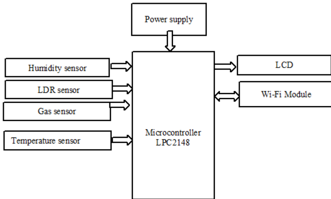
Fig 1: Block Diagram
