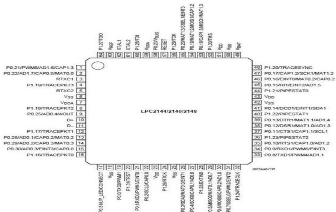
Fig2. LPC2148 Pin Diagram
