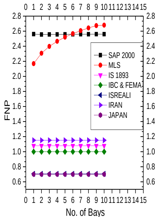
Fig 6 a) Variation of FNP for ten storey
