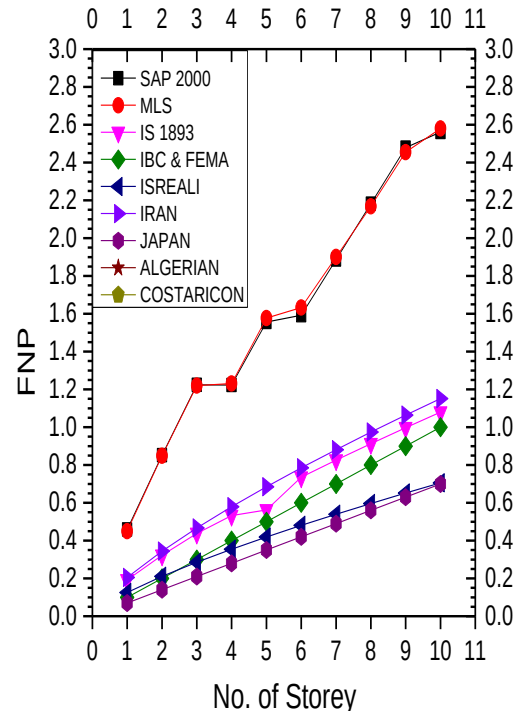
b) Variation of FNP for ten bay
