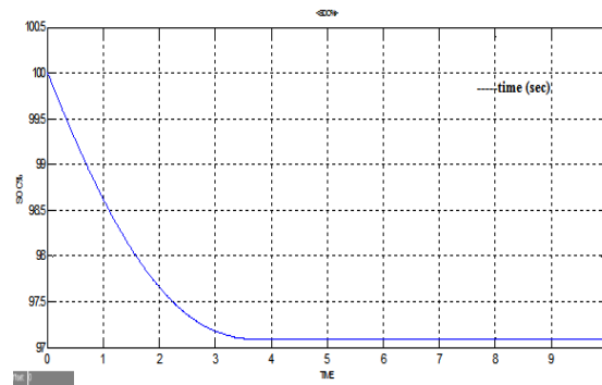
Figure 7(d): SOC% V/s Time of SC
