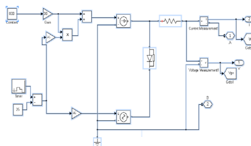
Figure 2: Simulation model of PV cell
