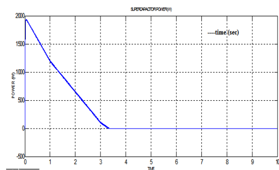
Figure 7(c): Power V/s Time of SC
