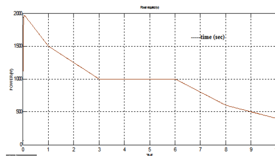
Fig 8(b): Power demanded V/s Time by load
