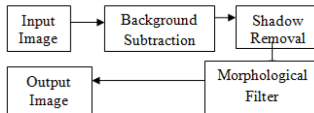
Figure 1: Silhouette Extraction
