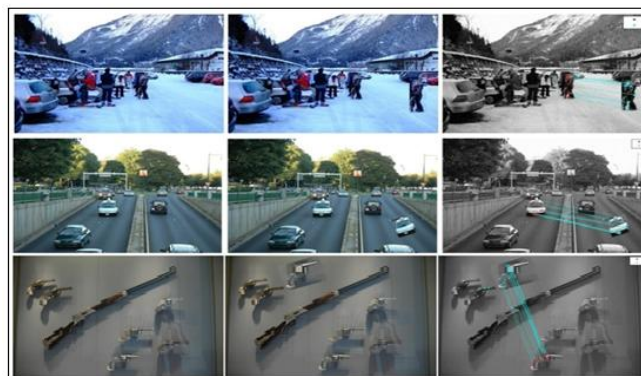
Figure 3:- Results of Hybrid DCT plus SIFT on Some Forged Images of Dataset MICC-F220.
