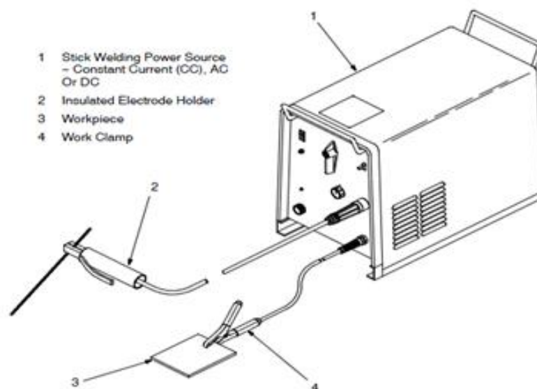
Figure 1: SMAW Machine
