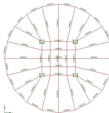
Fig. 5: Plan of Circular Building
