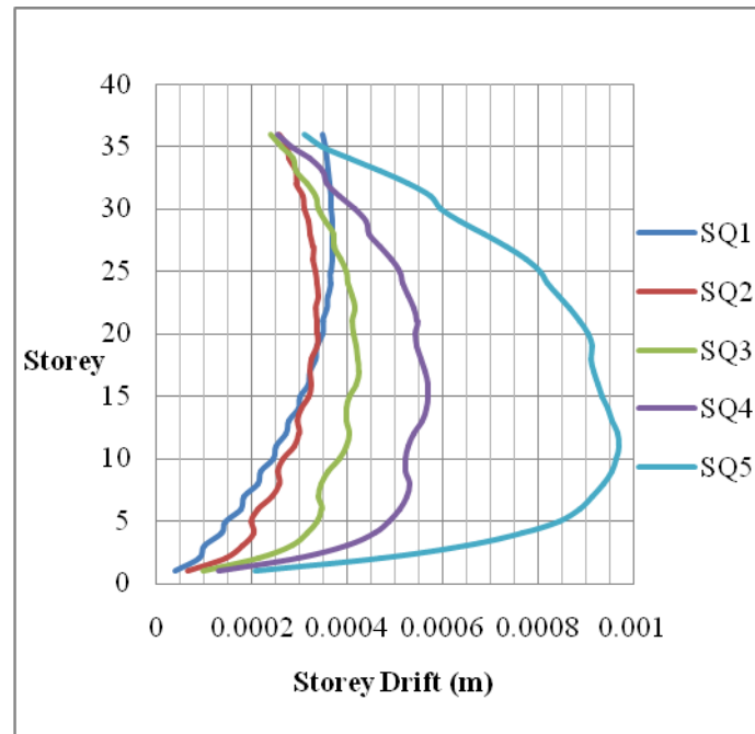
Fig. 8: Inter-Storey Drift Vs Storey for Square Models 1 to 5
