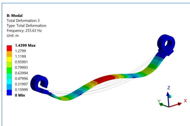
Fig.7. 2 nd Mode Shapes of Free Vibration of Composite Leaf Spring
