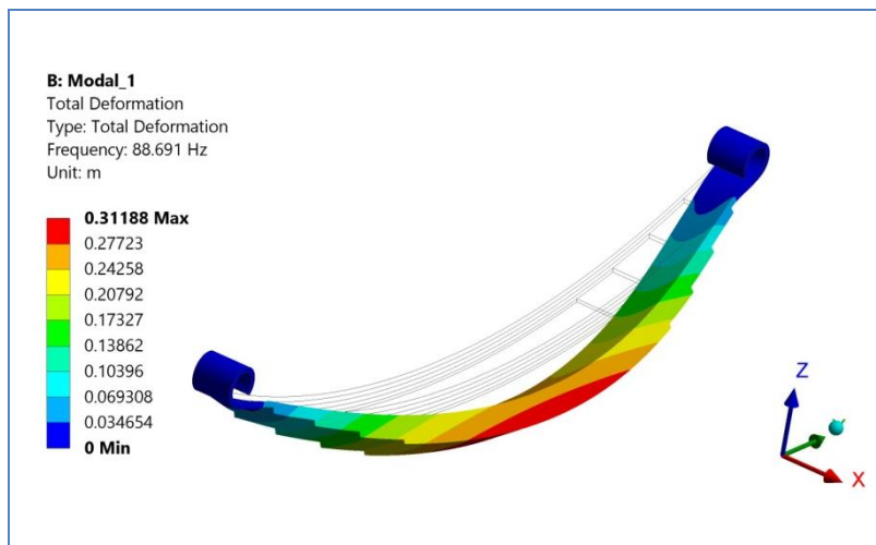
Fig.3. 1 st Mode Shapes of Free Vibration of Steel Leaf Spring
