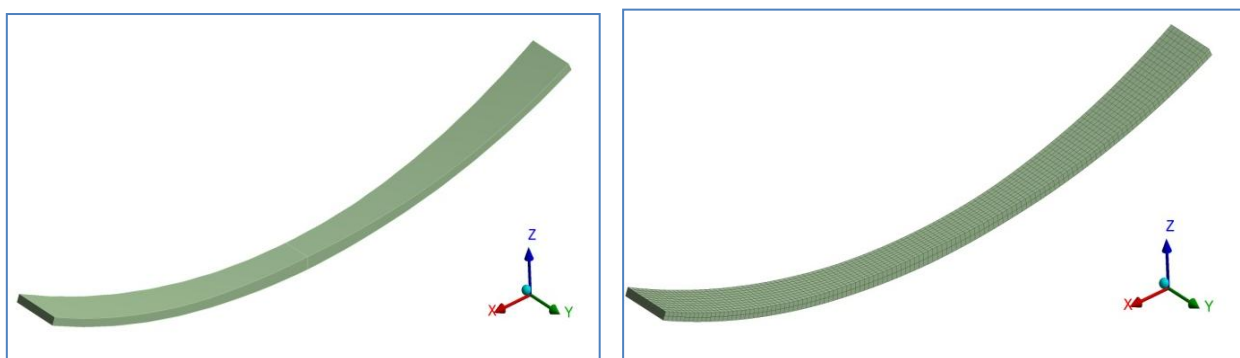
Fig.2 Cad Model and FE Model of Composite Leaf Spring
