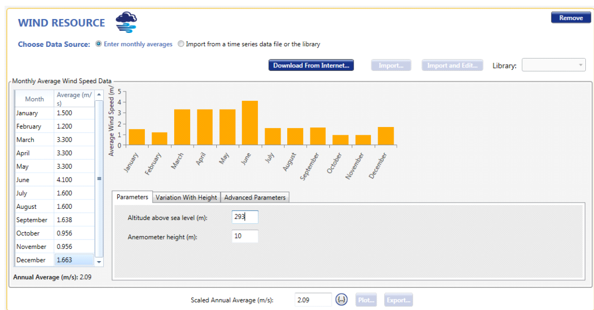
Fig 4. HOMER Data (Wind) for Our Visited Site.
