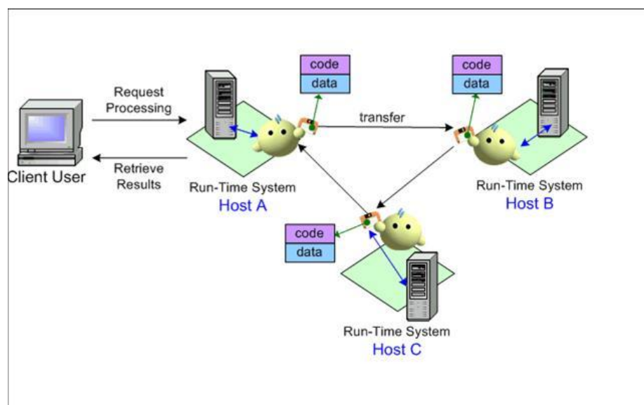
Figure 3. Cloud Environment
