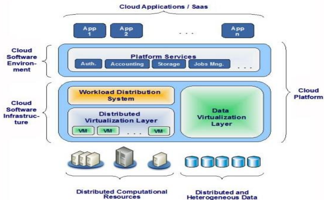
Figure 1. Cloud Architecture
