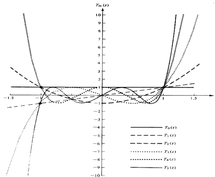
Fig 2: Chebyshev Polynomials T_0(x) , T_1(x) , T_2(x) , T_3(x) and T_4(x)
