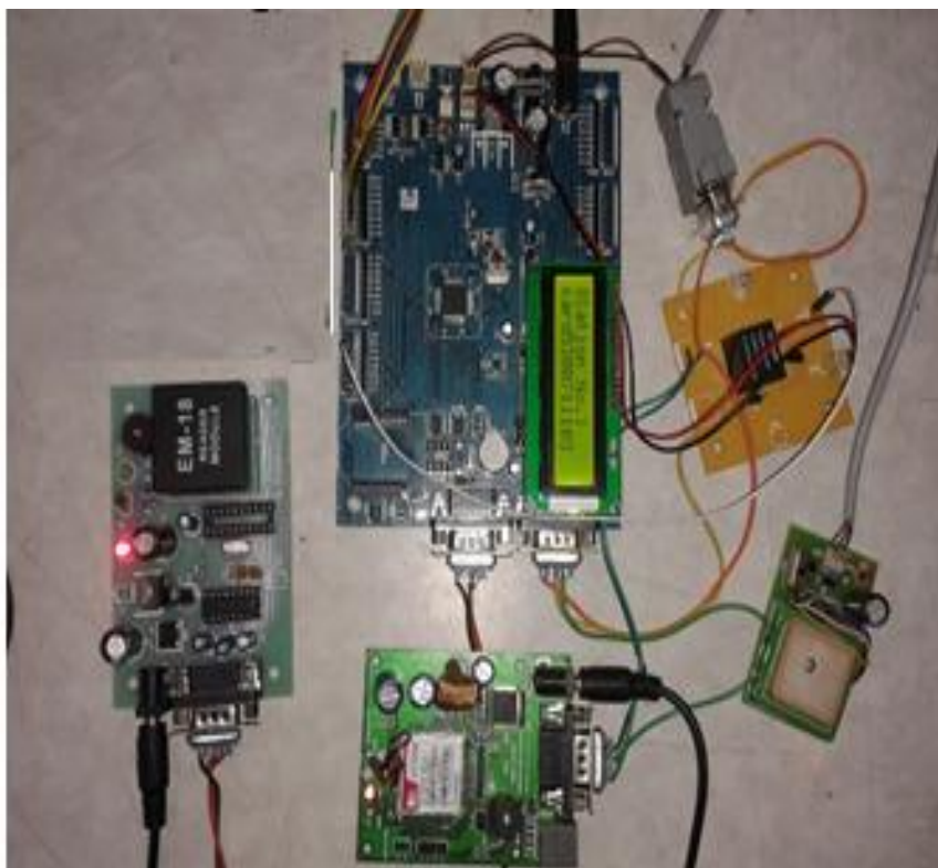
Fig 3: Overview of System Design Model
