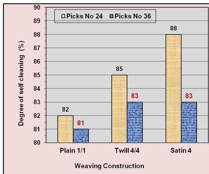
Figure 2: Effect of weaving construction and number of picks of PES/cotton blend fabric (constructed using 100 % cotton yarns in weft direction and 100 % PES yarns in warp direction) treated with \text{TiO}_2 NPs on degree of self-cleaning after 24 h exposure to sunlight
