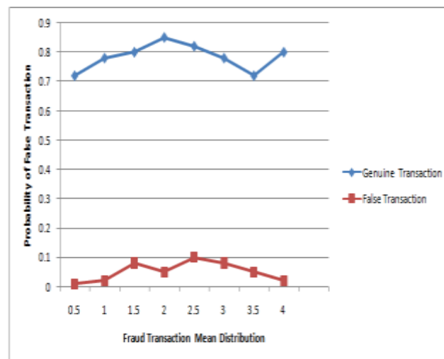
Figure 3. False Transaction
