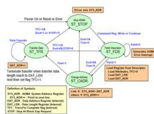
Fig 5.6: States of ADMA 2
