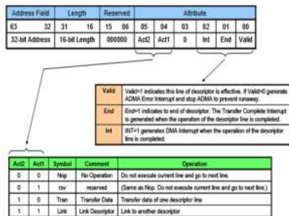
Fig 5.3: Example of Descriptor table
