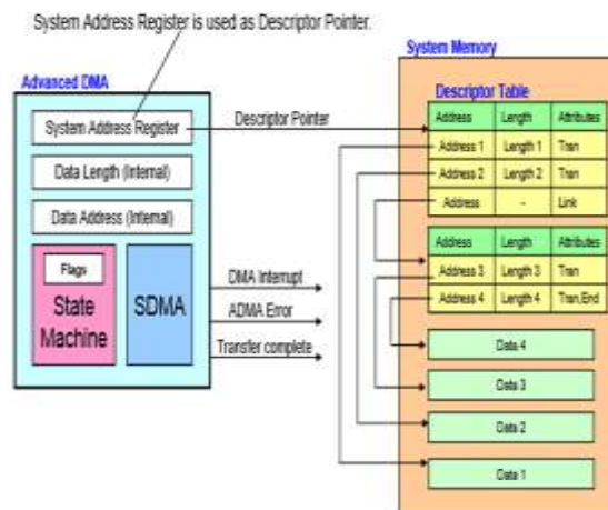
Fig 5.1: Block diagram of ADMA 2
