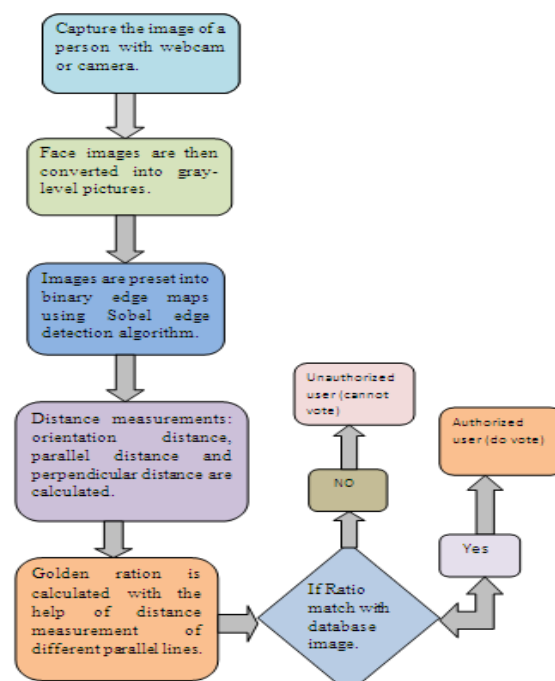
Figure1: Process Of Face Detection
