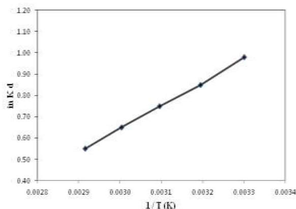
Figure 11: Van't Hoff plot
