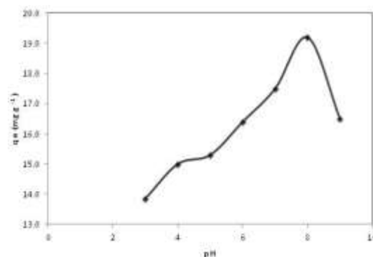
Figure 3: Effect of pH
