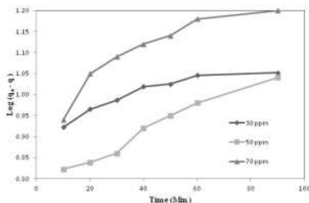
Figure 9: Pseudo first order kinetic model
