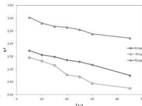
Figure 12: Intra-particle diffusion model
