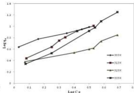
Figure 8: Freundlich adsorption isotherms
