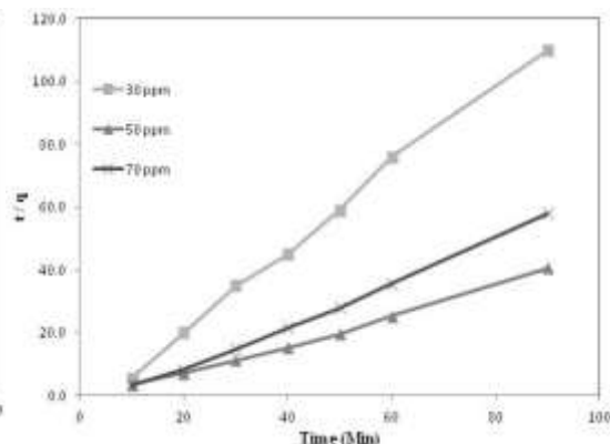
Figure 10: Pseudo second order kinetic model
