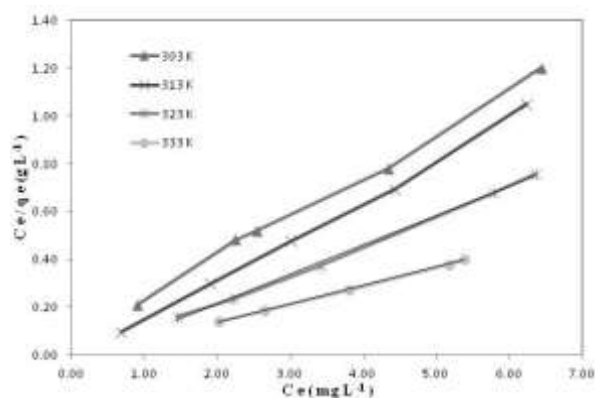
Figure 7: Langmuir adsorption isotherms
