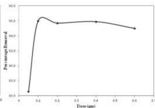
Figure 4: Effect of Adsorbent dose
