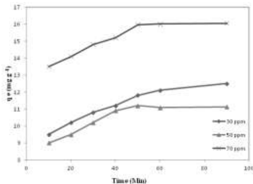
Figure 6: Effect of contact time
