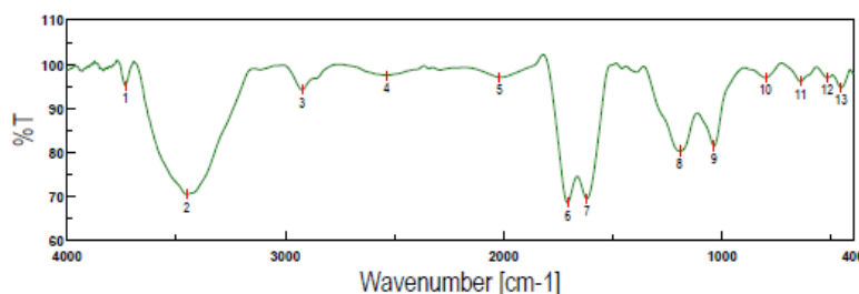
Figure 2: FTIR spectrum of TLAC
