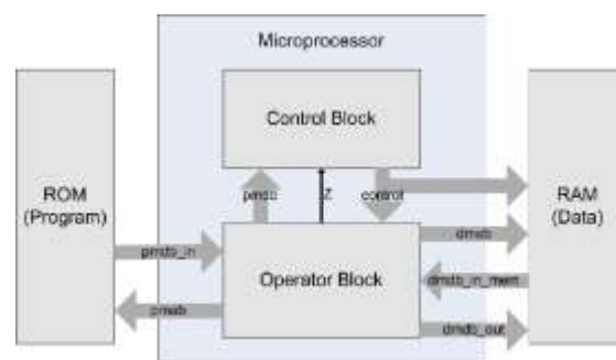
Fig. 2 - Internal Architecture
