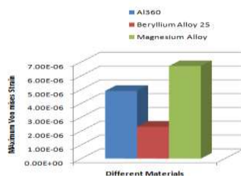
Figure 11: Max. von mises strain for different materials
