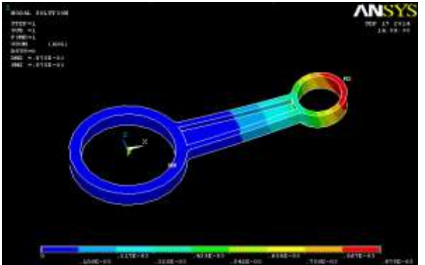
Figure 6: Displacement in connecting rod using beryllium alloy
