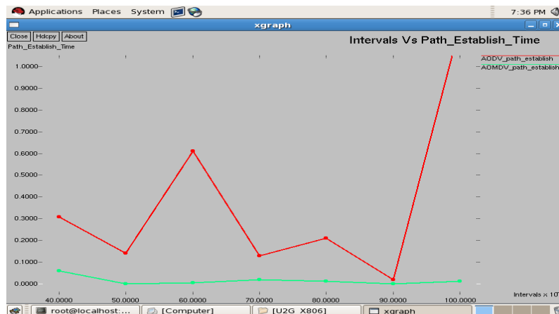
Fig. 7 Path establish time AODV vs AOMDV
