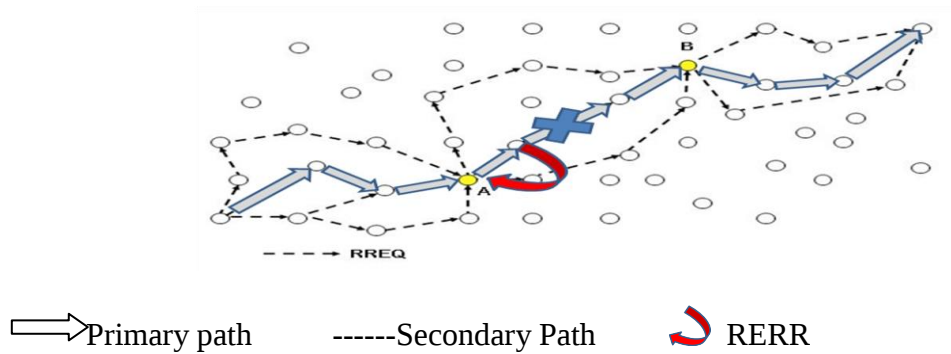
Fig. 5 Route maintenance process
