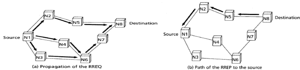
Fig. 1 Path in the AODV
