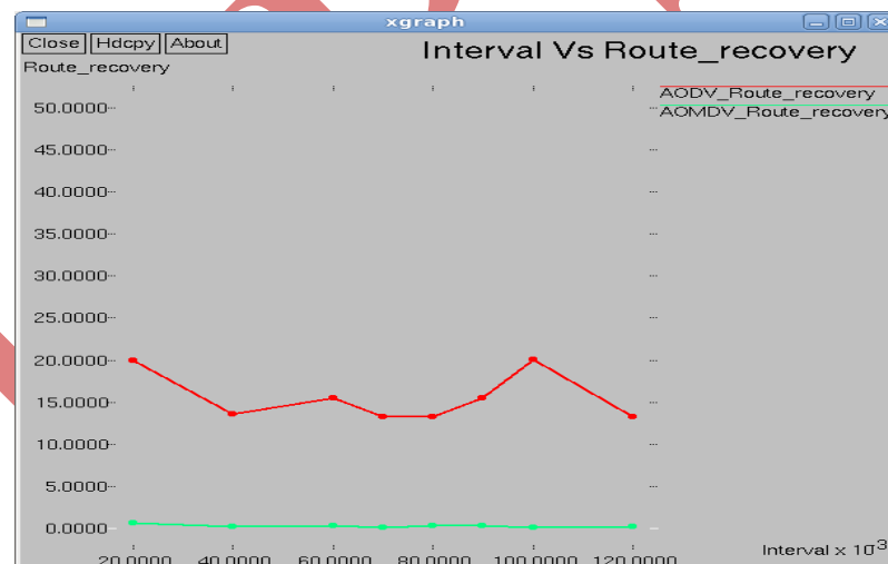
Fig. 8 Path recovery time
