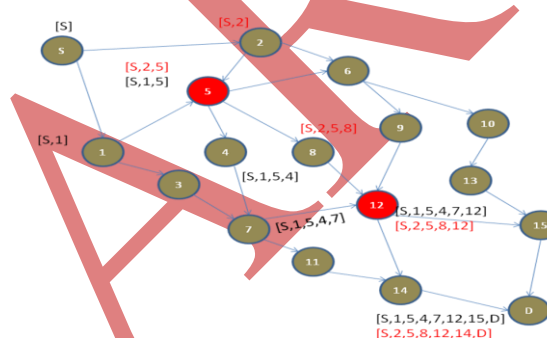
Fig. 4 Path creations from source to destination
