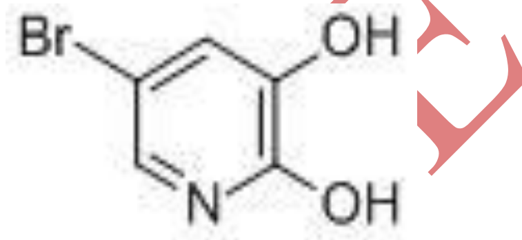
Figure: 1 Molecular Structure Of 5,2,3-BDHP
